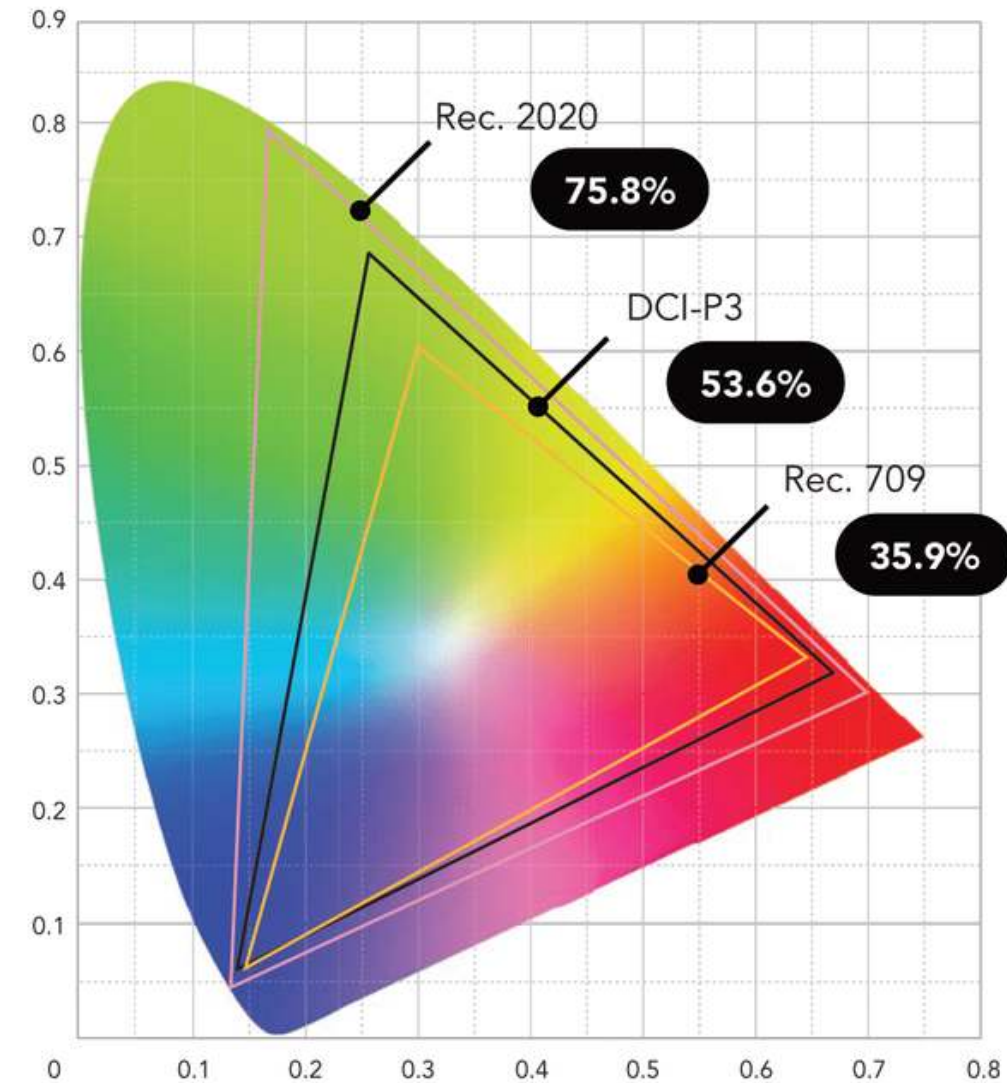
A color volume comparison of Rec. 2020, DCI-P3, and Rec. 709, and where they fall on the CIE 1931 chart. The CIE 1931 chart represents all the colors humans can see.
